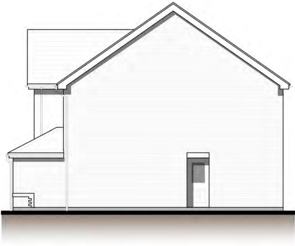
SIDE ELEVATION
